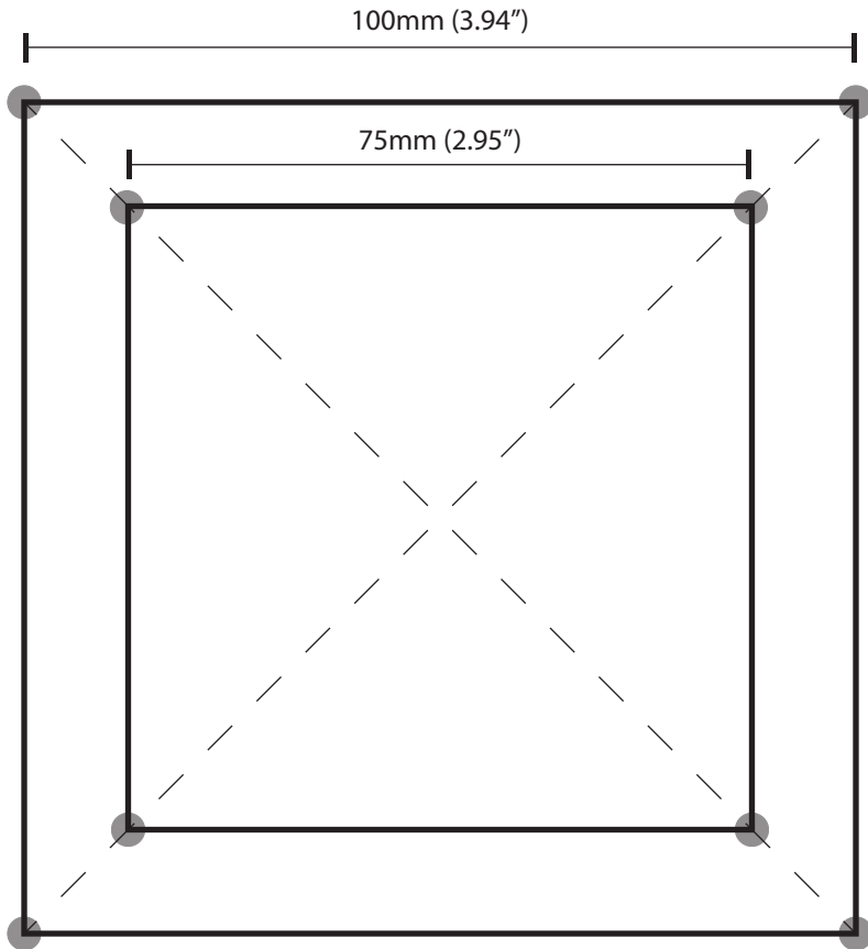
100mm / 75mm VESA Mounting Template (use 4mm screws)
